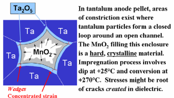
Figure 5. MnO 2 as contributing force to cracks.
