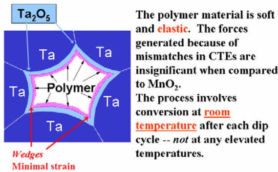
Figure 6. Compliant polymer minimizes forces.
