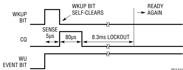
Figure 14. Wake-up Sequence
