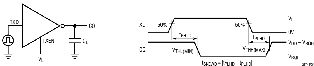
Figure 5. Driver Timing
