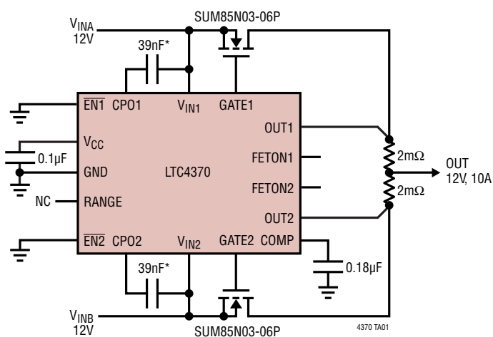
12V, 10A Load Share
