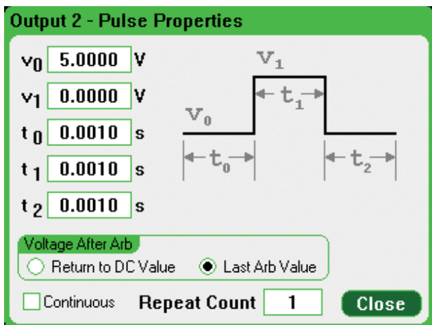
Figure 2a. N6705A pulse waveform configuration screen.
