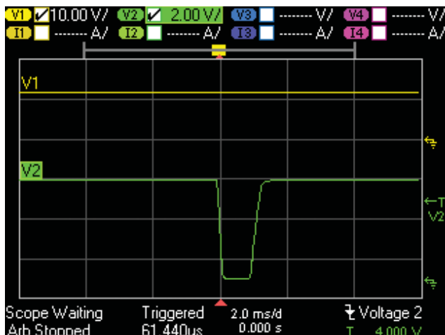
Figure 2b. Voltage waveforms on channels 1 and 2 in N6705A Scope View.
