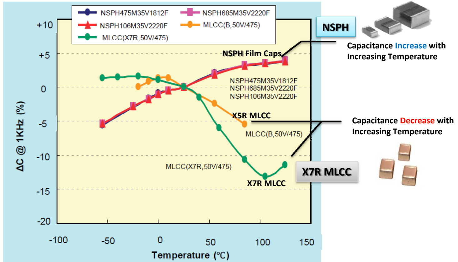
Typical Capacitance vs. Temperature (NSPH vs. MLCC)
