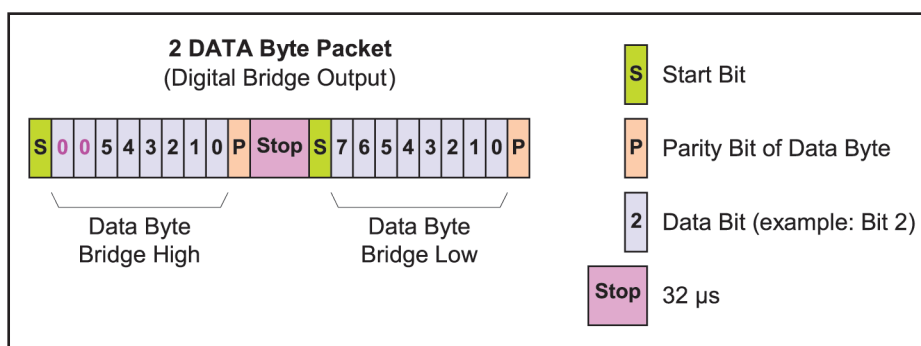
Figure 15: Digital Output Bridge Readings
